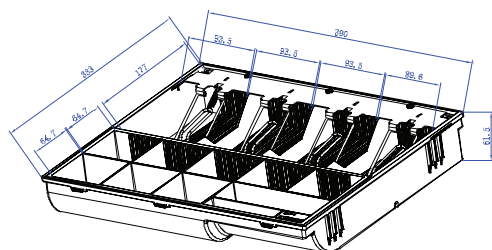
4-Bill Tray
