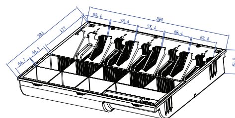
Unequal-5-Bill Tray
