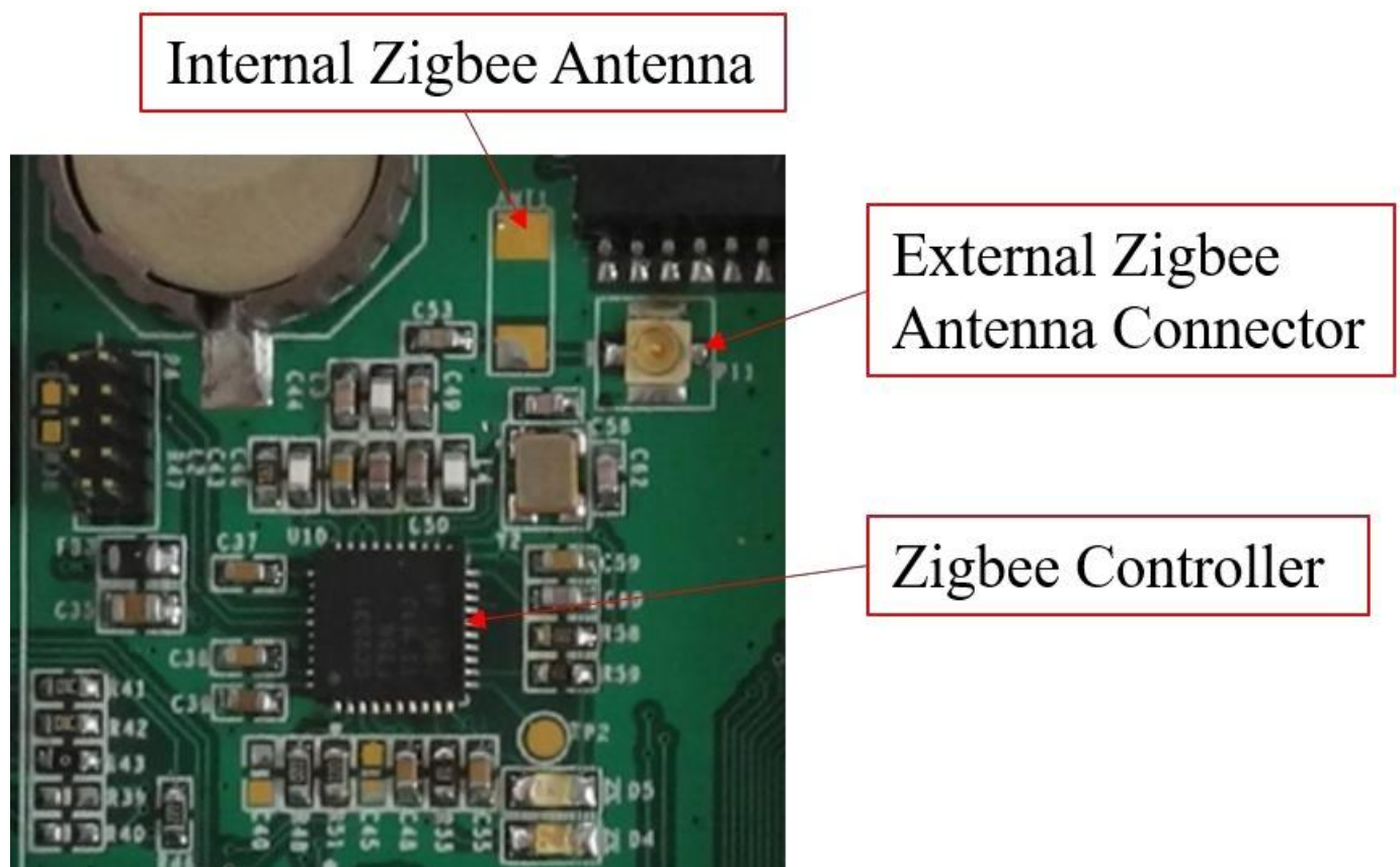
Figure 941: Zigbee controller
