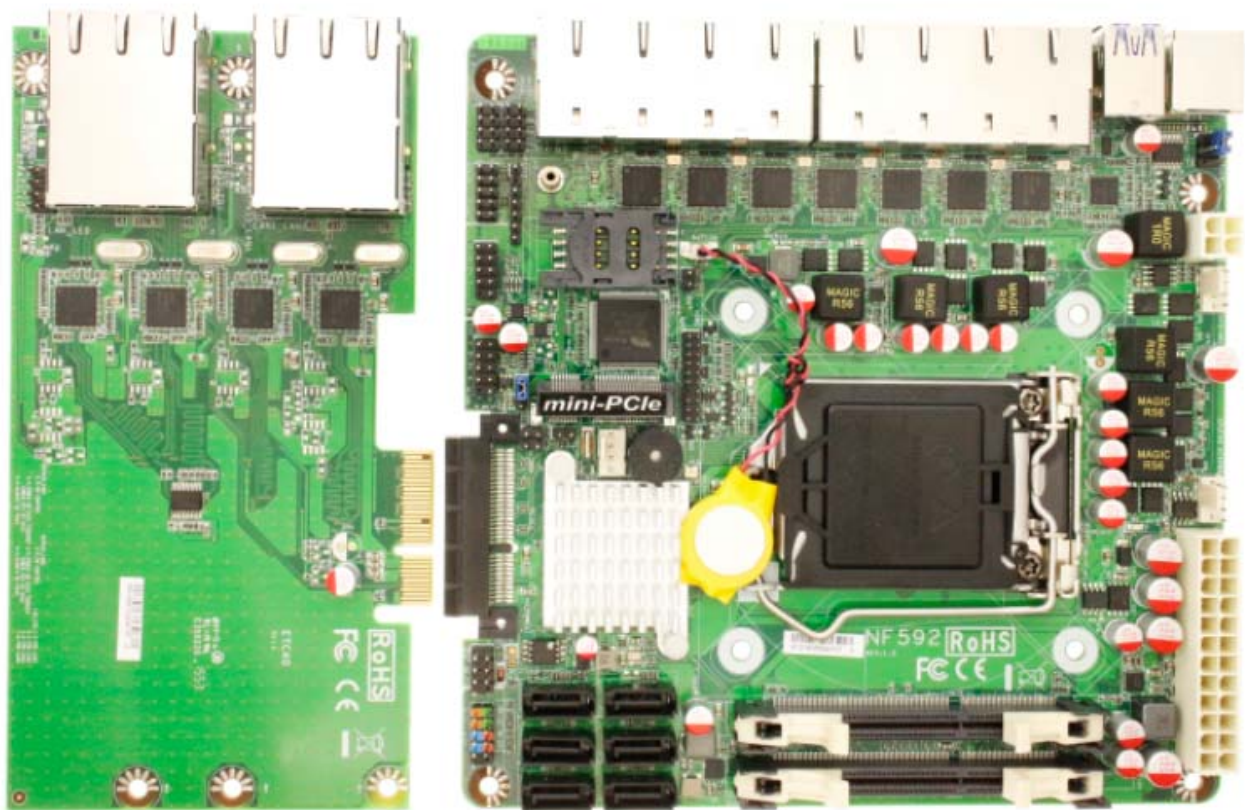
The figure shown JETC4B plug to the JNF592-Q170
