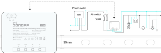
Installation Schematic
